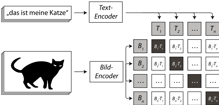
Text-Bild-Korrelation in CLIP
